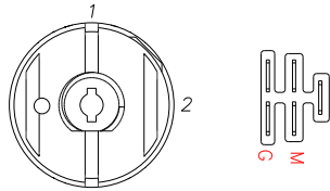
RECOMMENDED METAL PANEL MOUNTING HOLE (VIEW FROM BACK OF PANEL)
